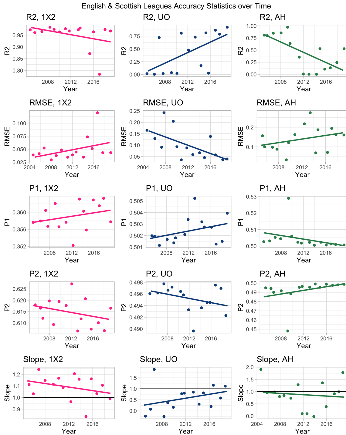
Figure 3.14: The variation of R^2 , RMSE, P_1 , P_2 , and the Slope over time in the English & Scottish leagues data
