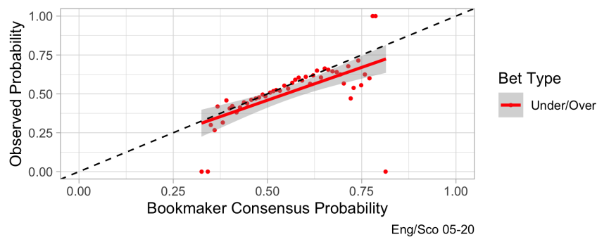
Figure 3.9: Consensus vs. observed probabilities on the English &amp; Scottish data, Under/Over 2.5 Goals market.
