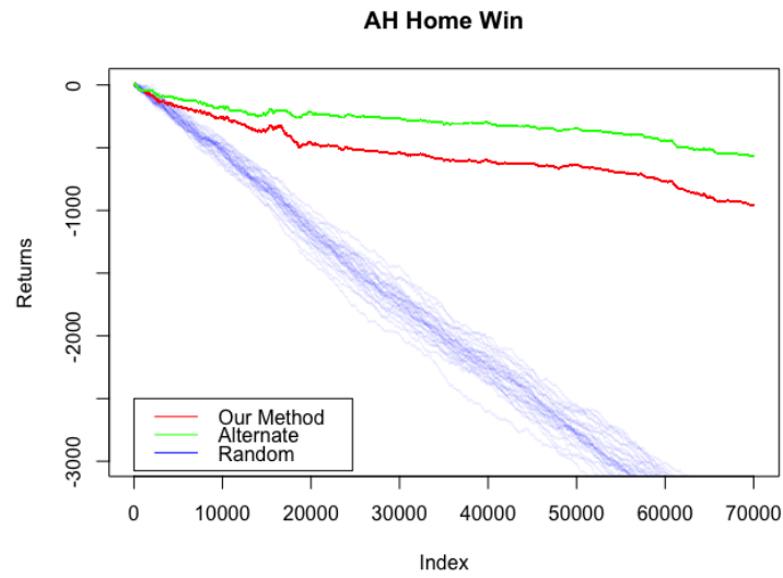
Figure 4.5: A line graph of the winnings of the random bet strategy in the AH Home Win market, compared to the proposed algorithm and the alternate method.
