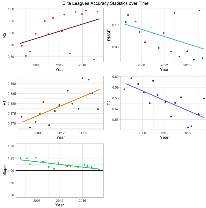
Figure 2.7: The variation of R^2 , RMSE, P_1 , P_2 , and Slope over time in the elite leagues data.
